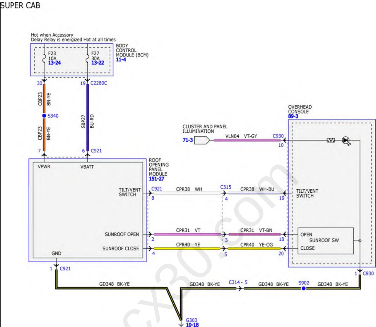
Fig 1: Roof Opening Panel System Wiring Diagrams (1 Of 3)
