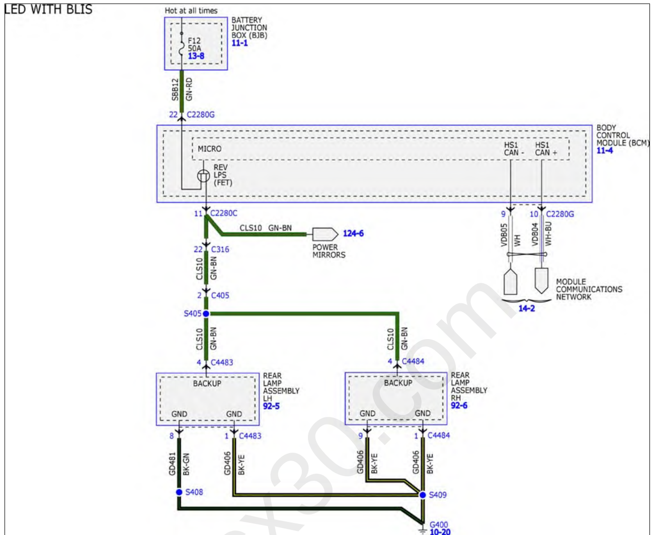
Fig 3: Reversing Lamps System Wiring Diagrams (3 Of 3)
