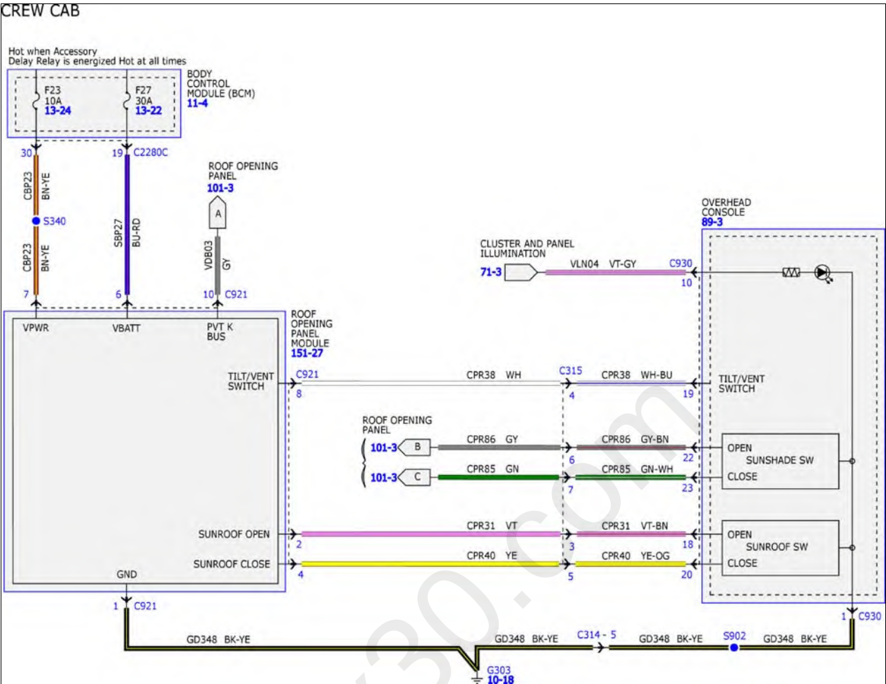
Fig 2: Roof Opening Panel System Wiring Diagrams (2 Of 3)
